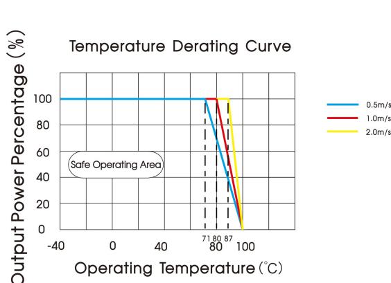
VCB4812EBO-100WR3 (Vin=48V)
