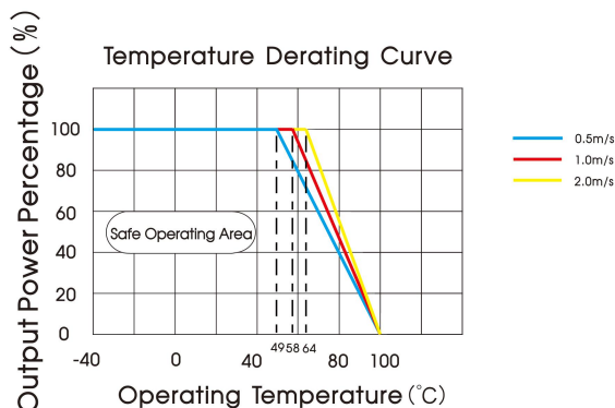
VCB4824EBO-100WR3 (Vin=48V)
