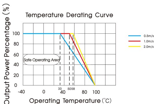
VCB4828EBO-100WR3 (Vin=48V)
