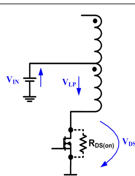
Figure 13 Self-adapting Positive Temperature Coefficient Rds(on)
