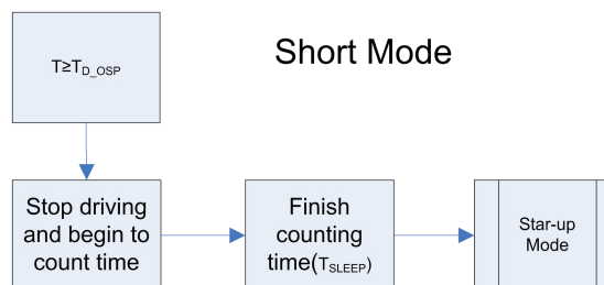
Figure 16 Flow Diagram of Short Mode
