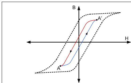
Figure 12 Magnetization Curve
