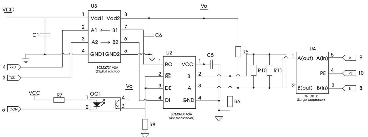
Figure 21 Application Circuit I
