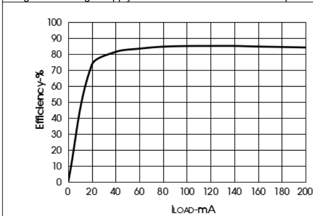
Figure 5 Efficiency and Load Current
