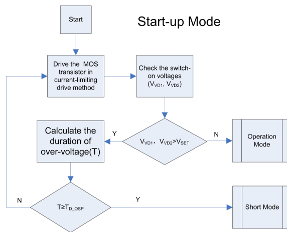
Figure 14 Flow Diagram of Start-up Mode
