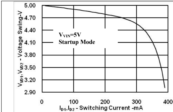
Figure 1 Drain Voltage of MOS Transistor VS. Switching Current of Primary Winding (Start Mode)
