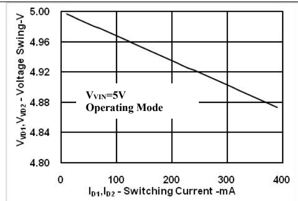
Figure 2 Drain Voltage of MOS Transistor VS. Switching Current of Primary Winding (Steady State Mode)
