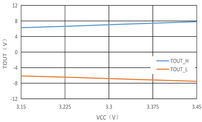
Figure 3. Transmitter Output Voltage High/Low VS V CC , R L =3 kΩ
