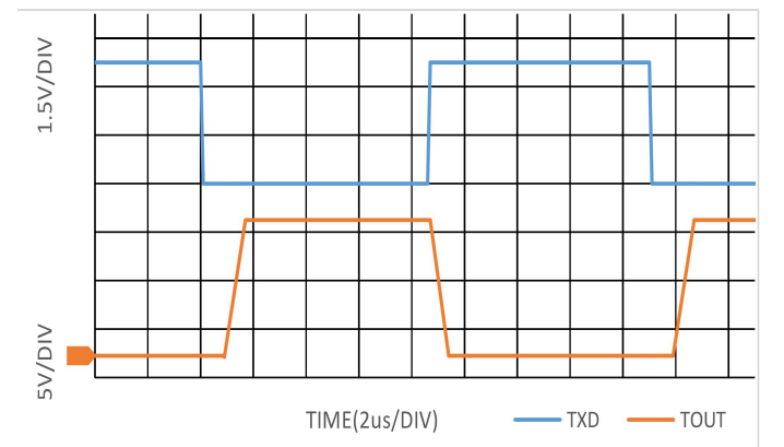
Figure 6. 120kbps Data Transmission (V CC =3.3V, R L =3 kΩ)
