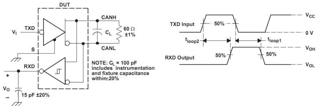
Figure 9. t(\text{LOOP}) Test Circuit and waveform
