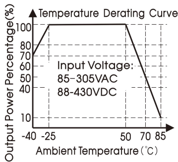
Natural air cooling 5 years design life
