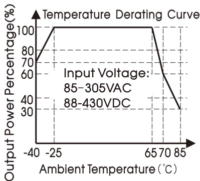
Forced cooling 5 years design life
