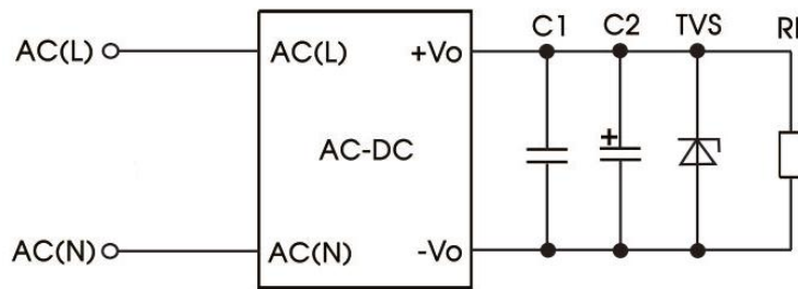
Fig. 1: Typical circuit diagram
