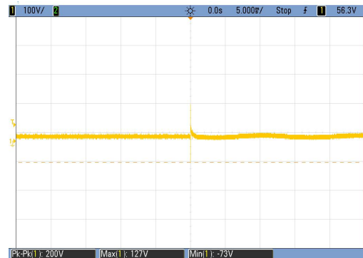
Output voltage waveform (0.12 KV)
